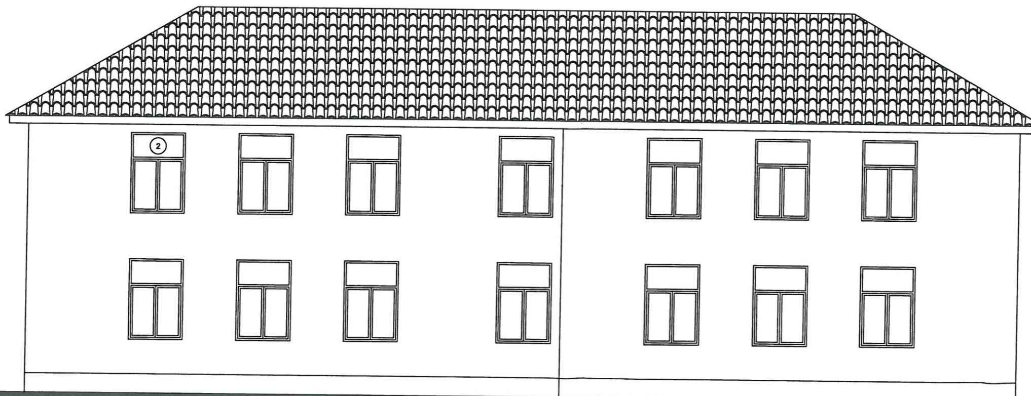
FATADA LATERALA STANGA - propusa
